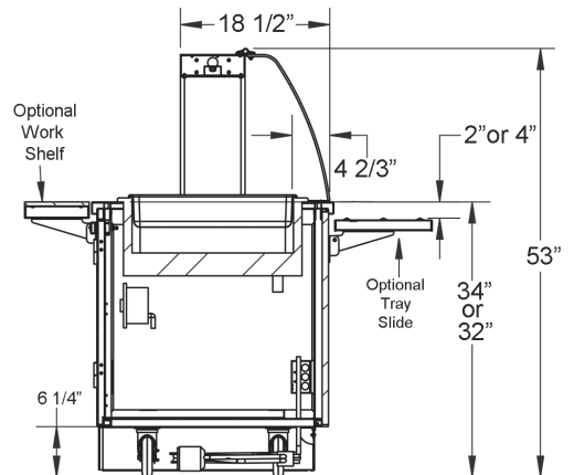
End View ▲
