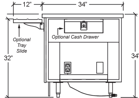
Model CSE30 Elevation
