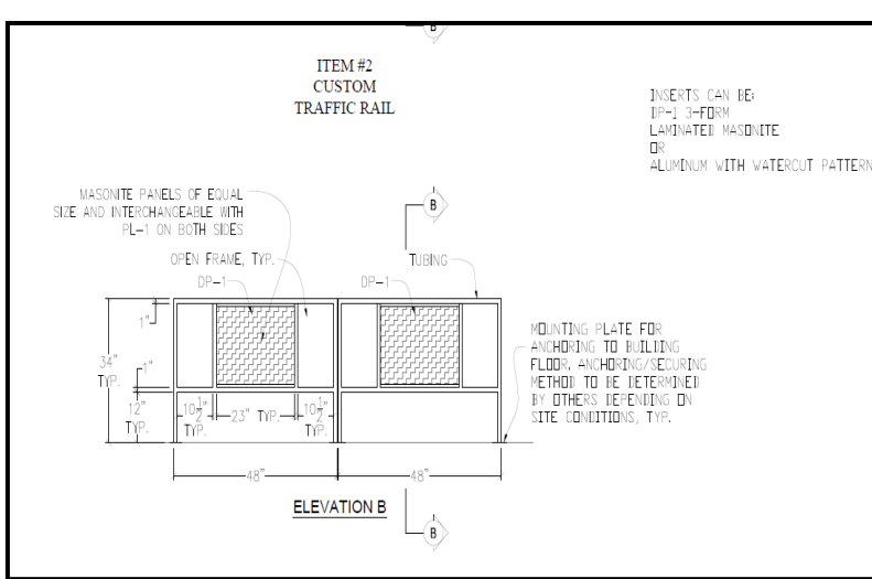
Elevation View ▲
